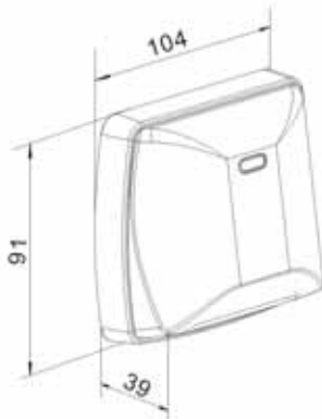
MJM Reader Dimensions:
