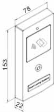
2700H Reader Dimensions:
