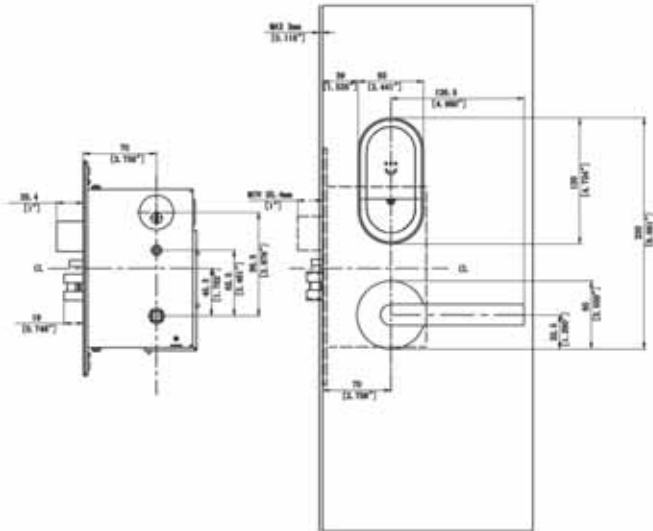
ANSI lockcase
